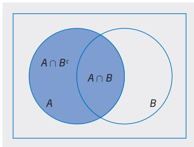
Figur 7.4 Venn-diagram for A = (A \cap B) \cup (A \cap B^c)
